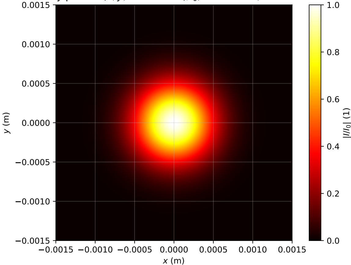
Intensity profile I(x, y, z = 0.000\text{m})/I_0 , P_{\text{in}}=0.2P_{\text{cr}} , artificial time
